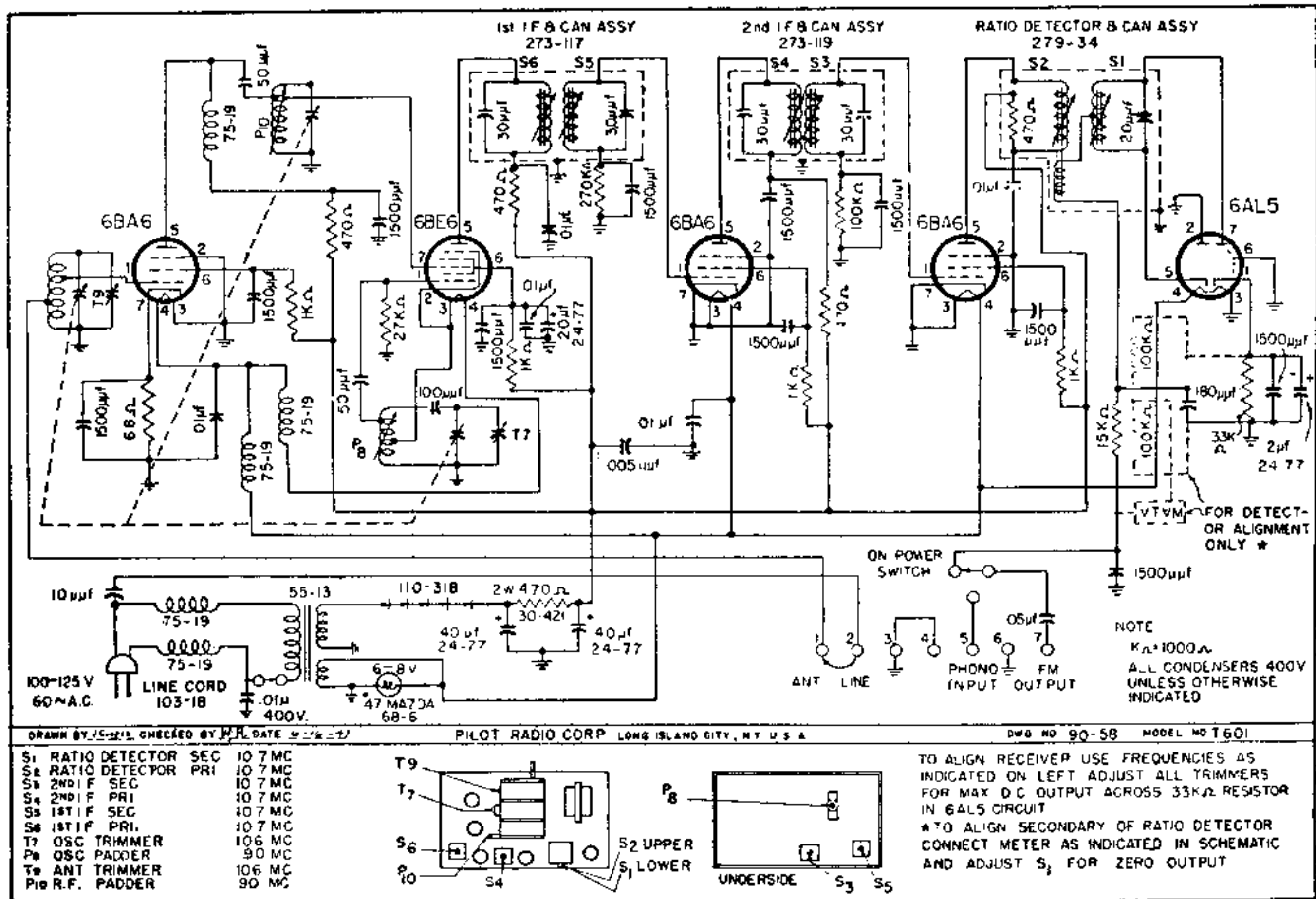
FIGURE 30 Schematic Diagram of FM Pilotuner.
