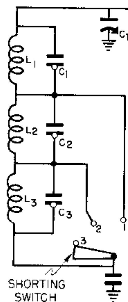
FIGURE 24 This is a typical use of a series coil connection in a preselector circuit. The shorting switch is part of the wave-band switch. When this switch is turned to position 1, it touches the contact of position 2 also; coils L_2 and L_3 are then shorted, leaving only L_1 to be tuned by condenser C_1 . When the switch is turned to position 2, coil L_3 is shorted; coils L_1 and L_2 are then in series and tuned by C_1 . When the switch is in position 3, all three coils are in series and tuned by C_1 . To align this set, you must turn the switch first to position 1 and adjust Trimmer C_1 , then to position 2 and adjust C_2 , and finally to position 3 and adjust C_3 .
