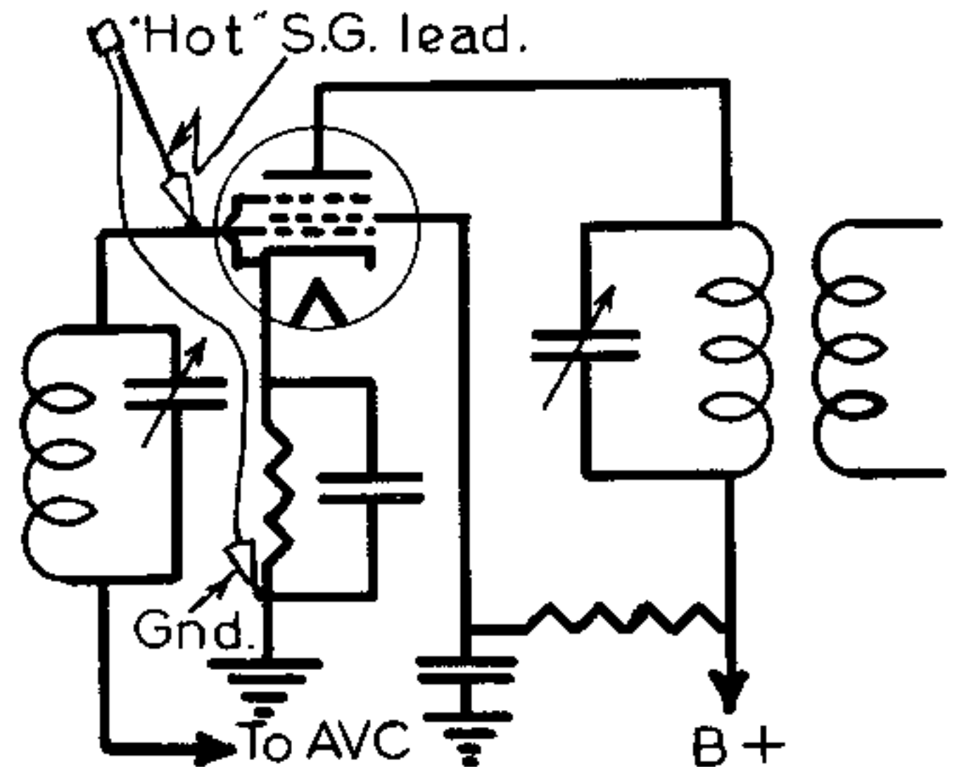
FIGURE 6 Typical I.F. Amplifier Circuit.
